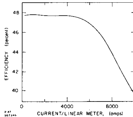
Fig. 3. Efficiency versus current, 200 kV beam energy.
