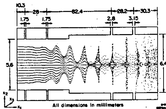
Fig. 2. Electron position-space distribution (not to scale) for the wiggler focused klystron with an initially laminar beam. RF ports are shown as gaps in the blocks. All dimensions are in mm.
